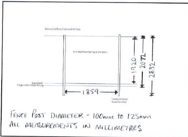
Image 2: Rabbit proof fence overlaying wire mesh fence
